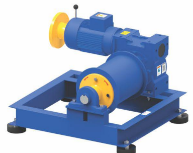
Dumbwaiter Machine
